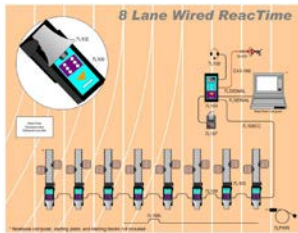
Wired Reactime system 8 lanes 1153020W price on request
